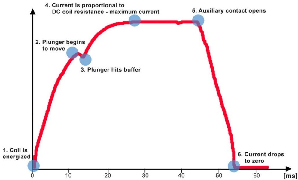
Figure 4. Typical coil current waveform
