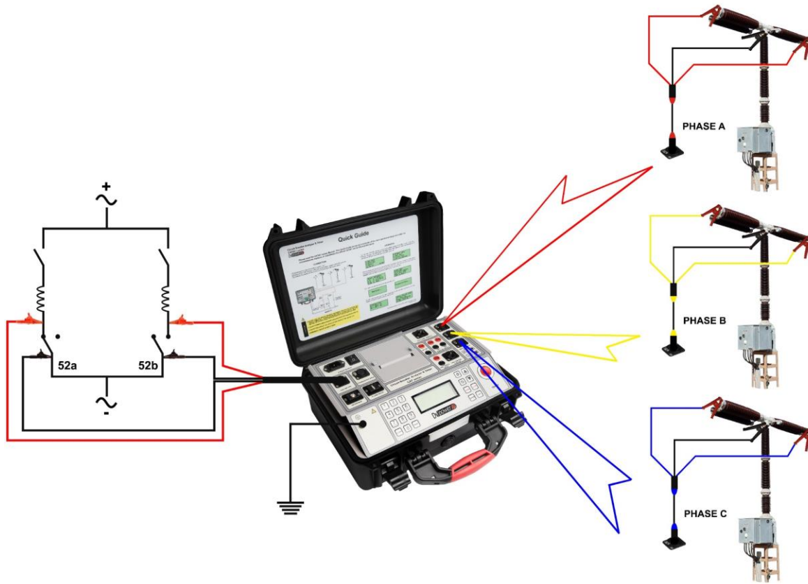
Figure 1: Connecting the main contact timing cables and auxiliary timing cables to a test object.
