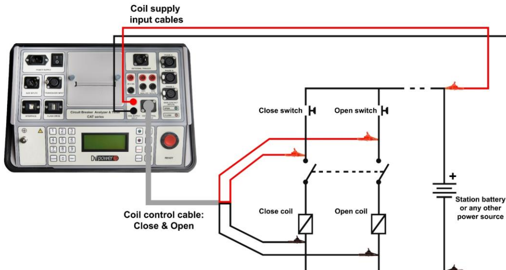
Figure 5. Connecting the coil control cables to circuit breaker control circuit
