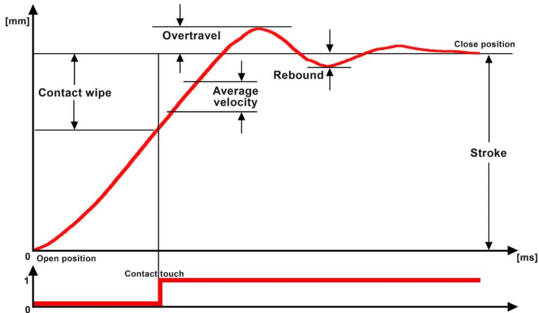
Figure 3. Travel curve and important travel parameters
